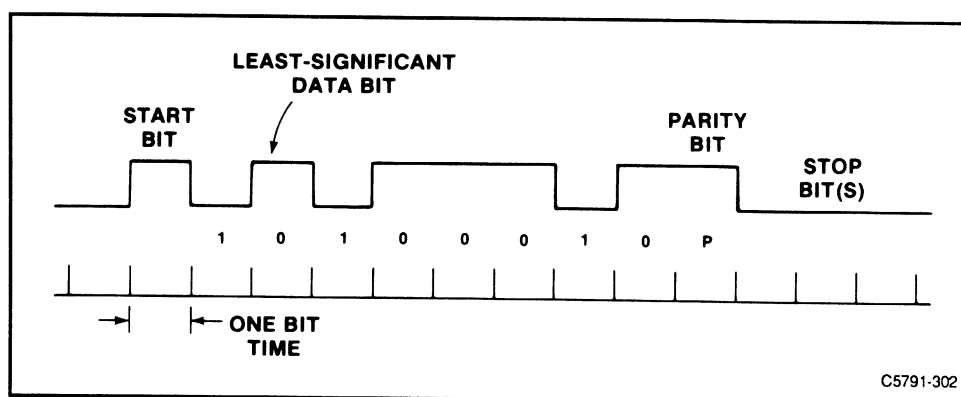
Figure 3-3. Asynchronous Serial Transmission.
