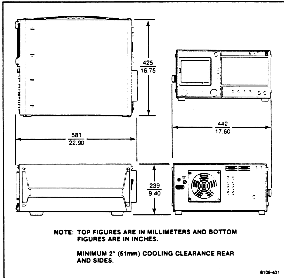
Figure 4-1. Bench Model.
