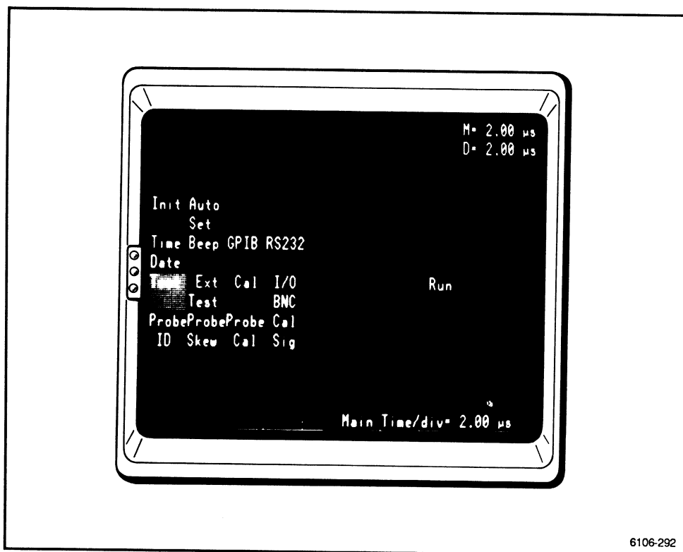
Figure 2-93. The Test menu.
