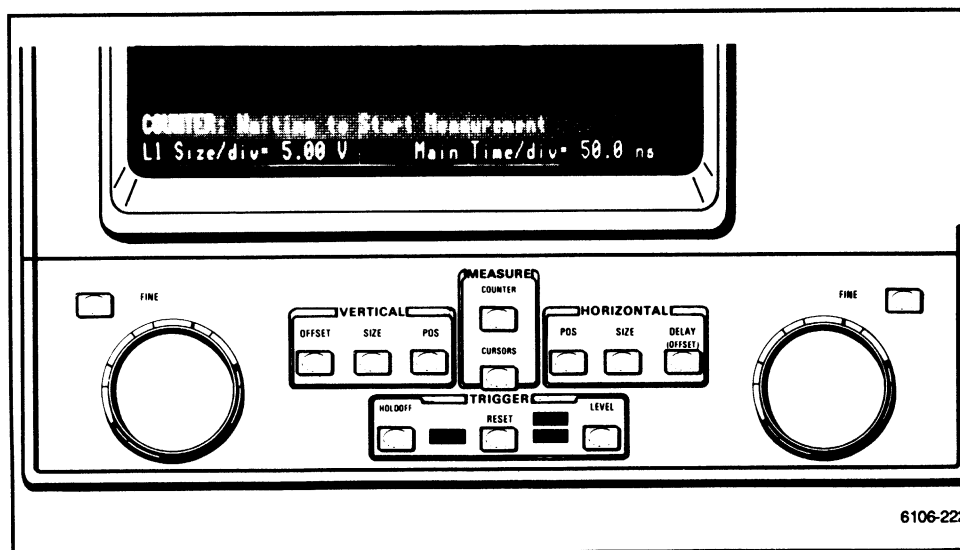
Figure 2-24. When the menu is Off, only the prompting and knob setting line appears.
