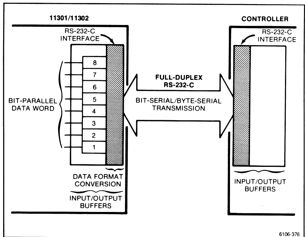
Figure 3-20. 11301/11302 RS-232-C Data Transfer.
