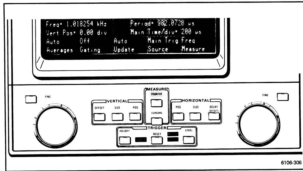
Figure 2-107. Counter/Timer menu.
