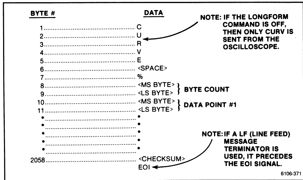
Figure 3-12. Binary Transfer Operation.
