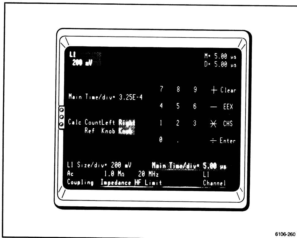
Figure 2-60. The NUMERIC ENTRY menu with a relative reference value set.
