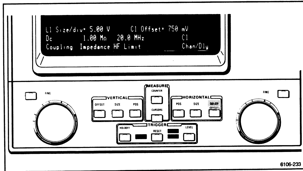
Figure 2-35. The right control knob is assigned to supply the offset for C1 even though it cannot be displayed vertically.
