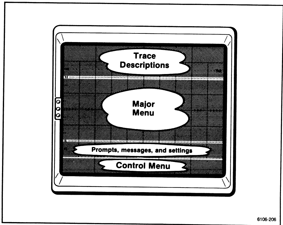
Figure 2-20. Display Format.
