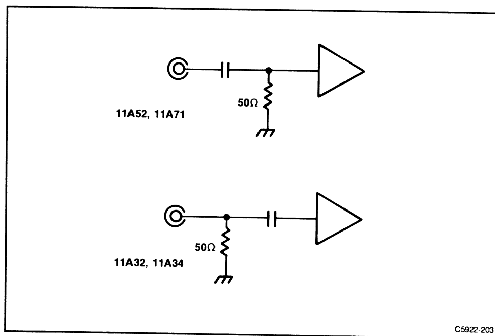
Figure 2-1. Location of AC coupling capacitors in plug-in amplifiers.
