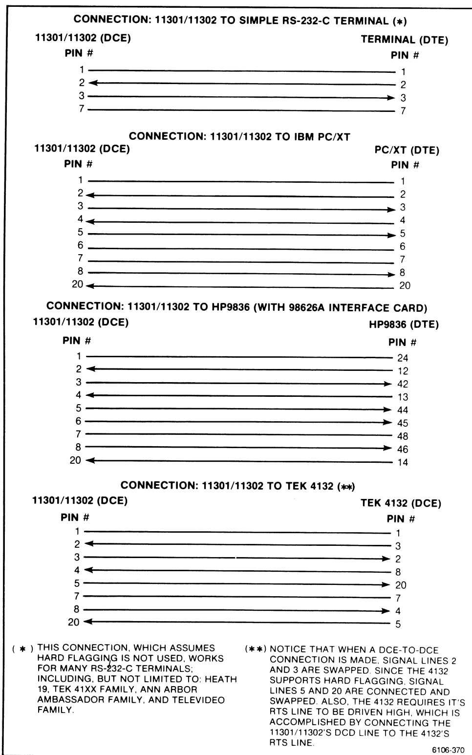
Figure 3-11. Examples of RS-232-C Connections.
