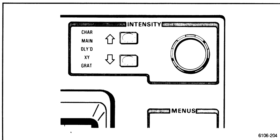
Figure 2-4. INTENSITY controls.
