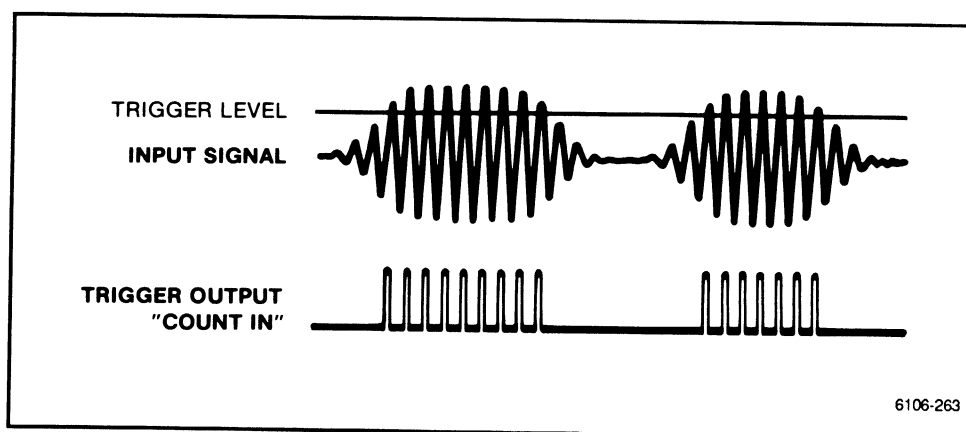
Figure 2-65. Trigger View trace shows pulses derived from two bursts of different durations.
