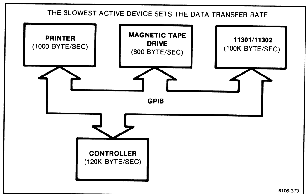
Figure 3-17. System Limitations On Data Transfer Rates.
