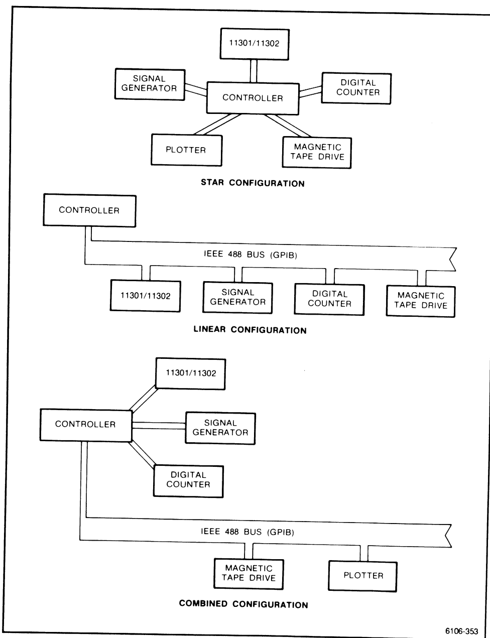
Figure 3-4. GPIB System Configurations.
