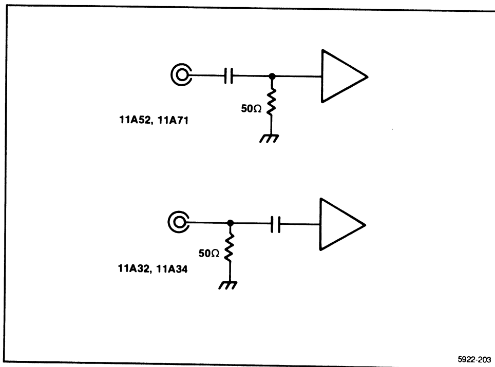
Figure 2-1. Location of AC coupling capacitors in plug-in amplifiers.
