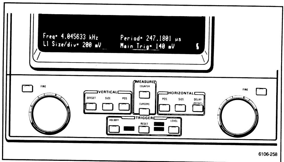
Figure 2-58. Alternate presses of the COUNTER button preserve the knob setting and results.
