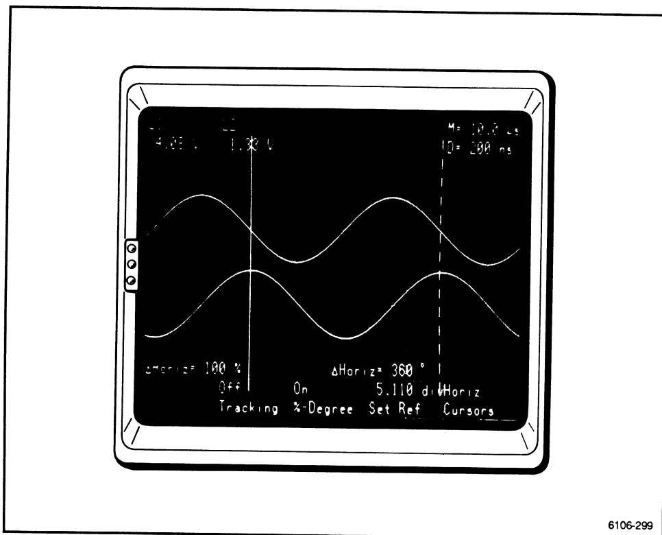
Figure 2-100. Selecting one cycle with the Horizontal Cursors.
