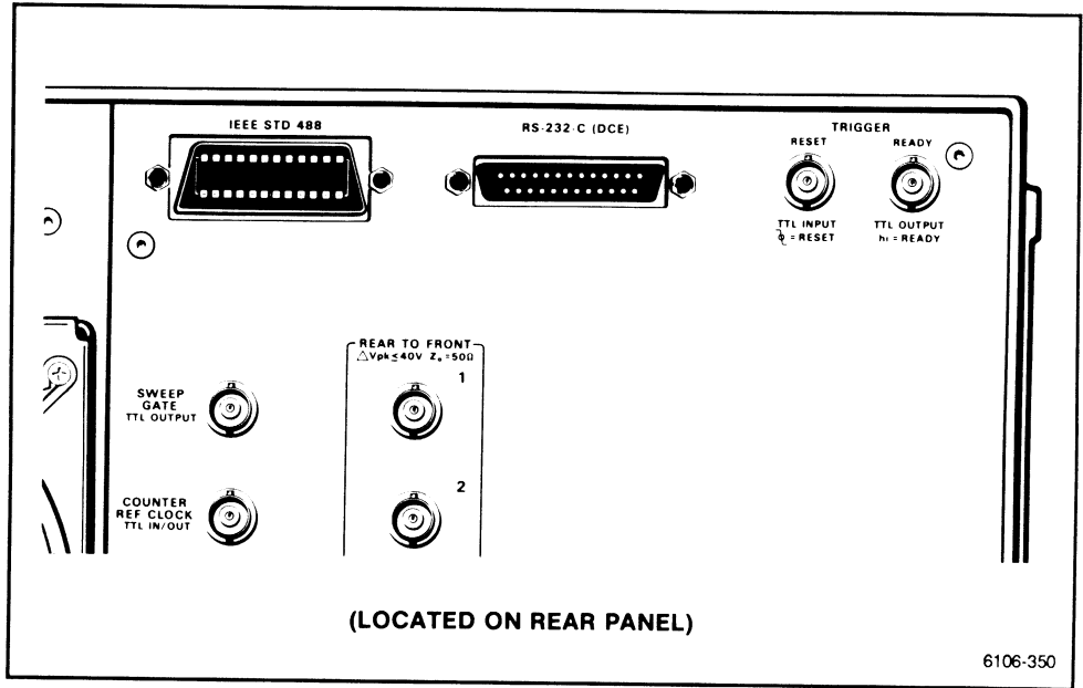
Figure 3-1. GPIB & RS-232-C Ports (Rear Panel View).
