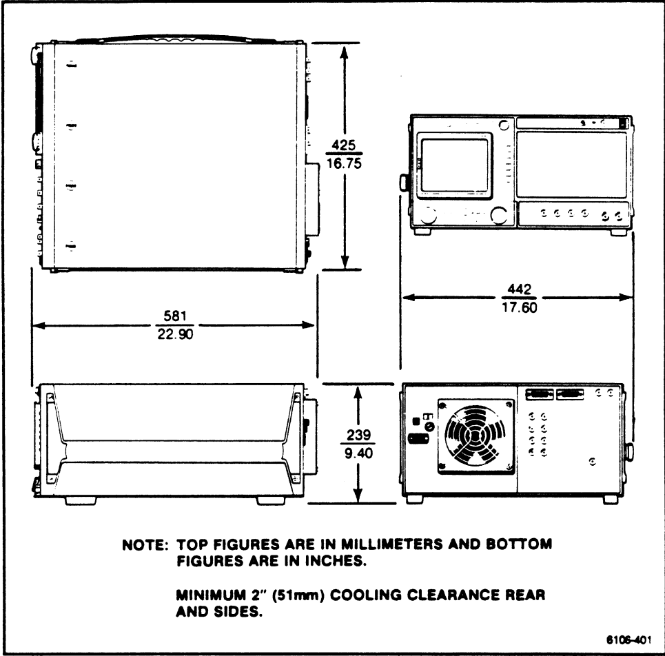
Figure 4-1. Bench Model.
