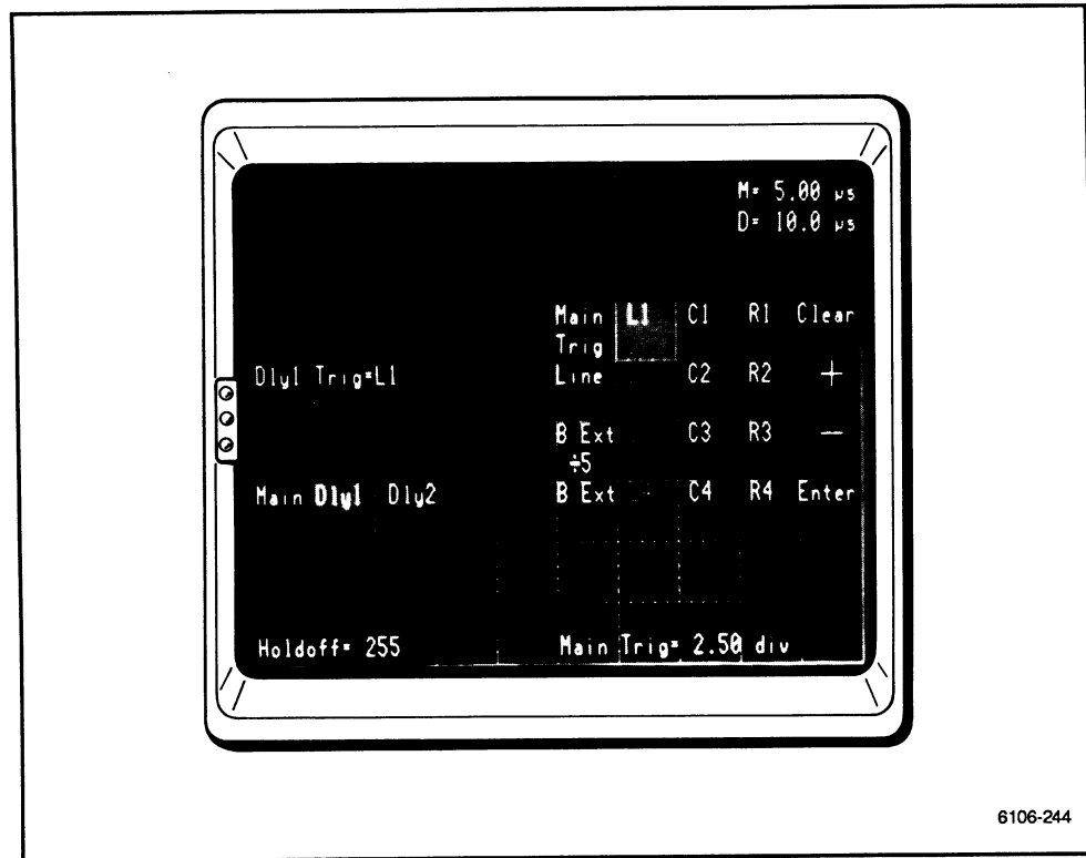
Figure 2-45. This example shows the selections (right half of menu) available for the Dly1 trigger source. The Dly2 trigger source menu offers the same selections.
