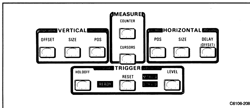
Figure 2-9. Control-menu buttons.
